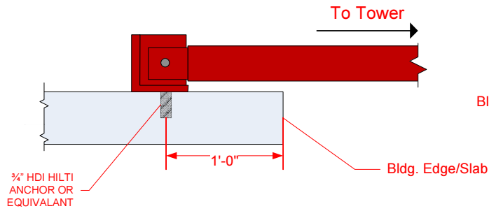
SIDE VIEW/SECTION N.T.S.
