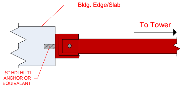
SIDE VIEW/SECTION N.T.S.
