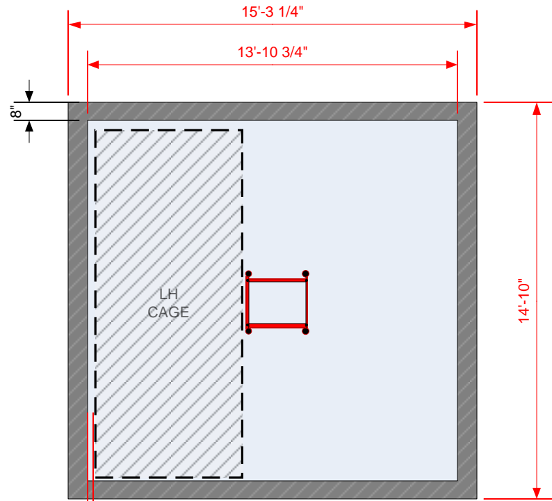
PLAN VIEW @ TOP OF CARS N.T.S.
