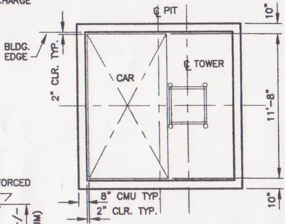
PLAN @ TOP OF CARS
